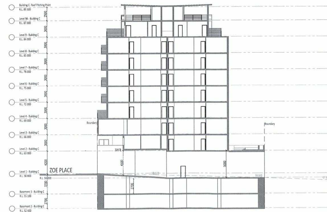
SECTION F-F
