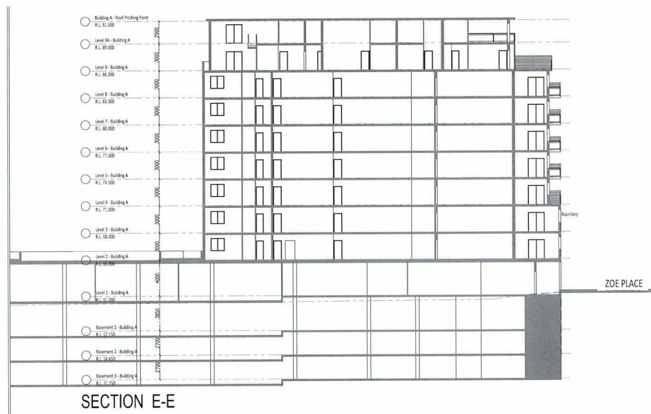
SECTION E-E
