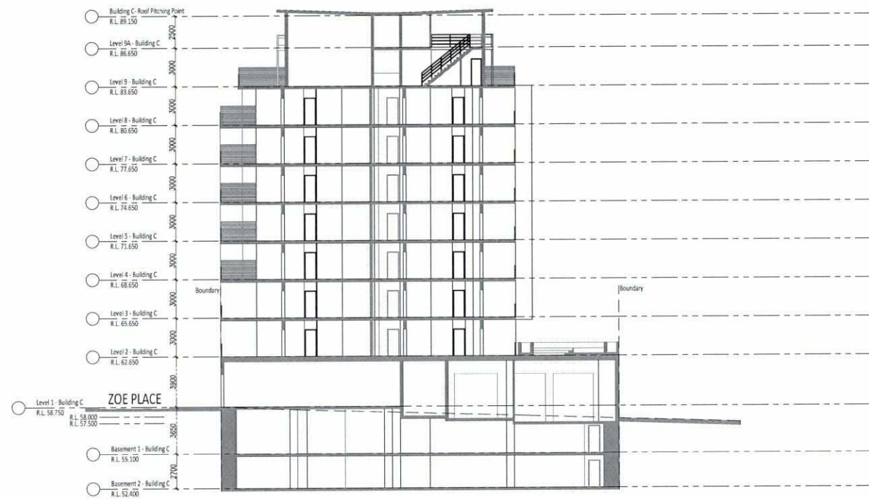
SECTION C-C
